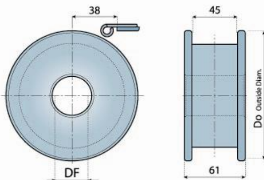
整体式从动轮 (机加工) SINGLE-PIECE IDLER WHEELS (MACHINED)
