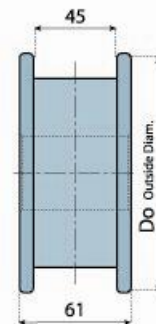
整体式从动轮 (机加工) SINGLE - PIECE IDLER WHEELS (MACHINED)
