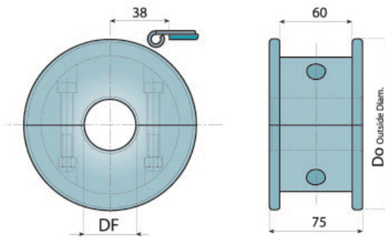
整体式主动轮 (机加工) SINGLE-PIECE SPROCKETS (MACHINED)
