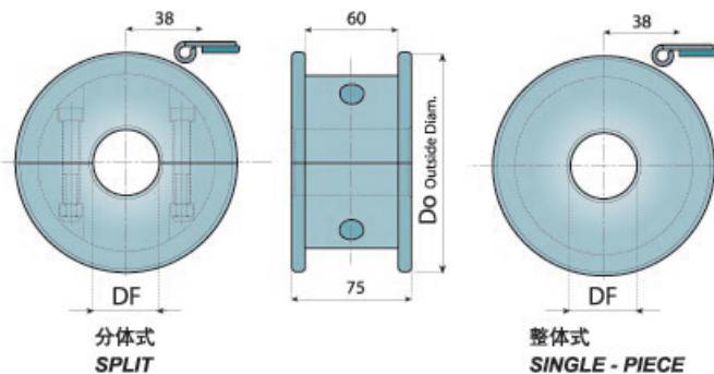
整体式 SINGLE - PIECE
