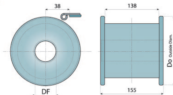
整体式从动轮 (机加工) SINGLE - PIECE IDLER WHEELS (MACHINED)
