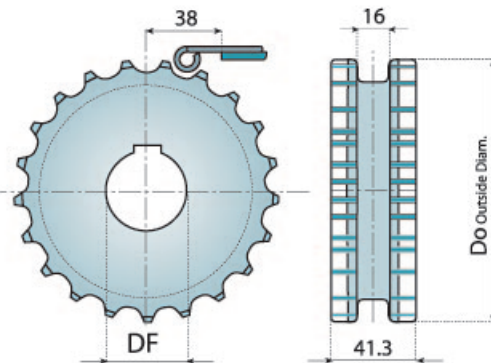
整体式主动轮 (机加工) SINGLE - PIECE SPROCKETS (MACHINED)
