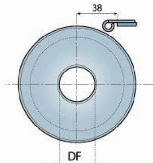
整体式从动轮 (机加工) SINGLE - PIECE IDLER WHEELS (MACHINED)
