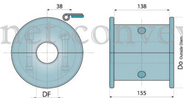
分体式从动轮 (机加工) SPLIT IDLER WHEELS (MACHINED)
