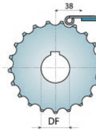
整体式 SINGLE - PIECE
