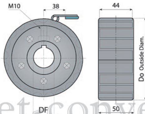
整体式主动轮 (注塑) SINGLE-PIECE SPROCKETS (INJECTION)
