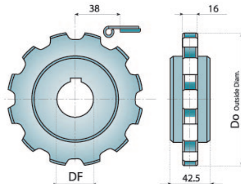
整体式主动轮 (机加工) SINGLE-PIECE SPROCKETS (MACHINED)
