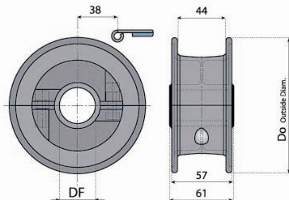
分体式从动轮 (注塑) SPLIT IDLER WHEELS (INJECTION)
