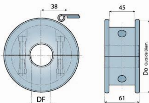
分体式从动轮 (机加工) SPLIT IDLER WHEELS (MACHINED)
