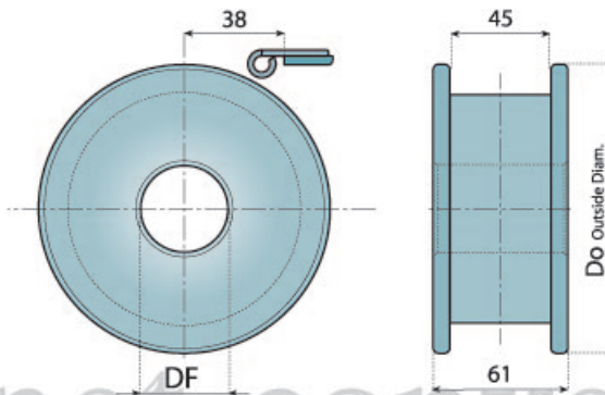
整体式从动轮 (机加工) SINGLE-PIECE IDLER WHEELS (MACHINED)
