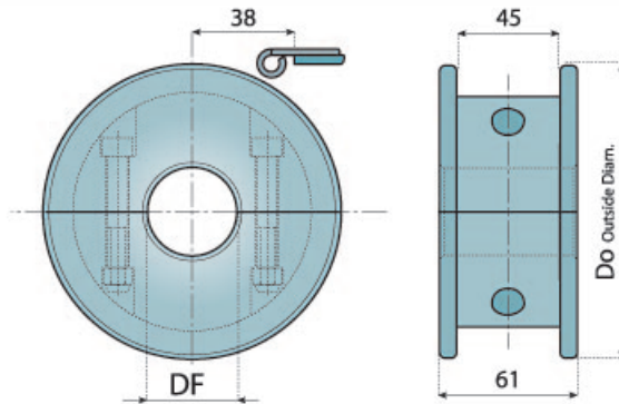
分体式从动轮 (机加工) SPLIT IDLER WHEELS (MACHINED)
