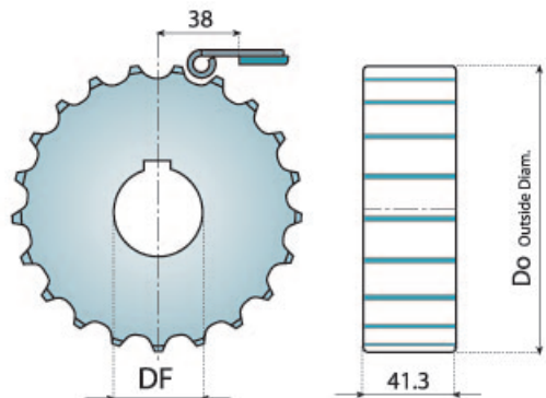
整体式主动轮 (机加工) SINGLE-PIECE SPROCKETS (MACHINED)
