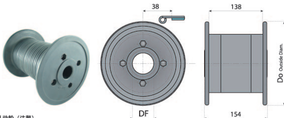
从动轮 (注塑) IDLER WHEELS (INJECTION)
