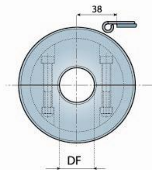
分体式从动轮 (机加工) SPLIT IDLER WHEELS (MACHINED)
